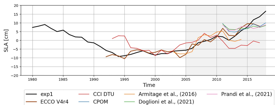
Figure 1. Sea level anomalies annual time series (1980–2018) in the Beaufort Gyre Region box of (black curve) the control run exp1 and of altimetry products: (red curve) CCI DTU (Rose et al., 2019), (blue curve) CPOM, (orange curve) Armitage et al. (2016), (green curve) Doglioni et al. (2021), (purple curve) Prandi et al. (2021), and (brown curve) the state estimate ECCO V4r4. Altimetry and ECCO V4r4 time series are shifted before plotting, using the model's time-averaged value over the overlap period of the data compared to exp1, to facilitate visual comparison. All time series are corrected from their respective global mean sea level and time mean. The period shaded in light gray corresponds to the period of interest 2005–2018.
