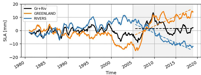
Figure 2. Monthly mean sea level anomalies time series in the Beaufort Gyre Region box with a 12-month running mean. The black curve represents exp1 minus CLIM (Gr + Riv), the orange curve exp1 minus exp2 (GREENLAND), and the blue curve exp2 minus CLIM (RIVERS). The dotted black, blue, and orange lines are the linear trends of their corresponding curves over 2005–2018. The gray shaded part highlights the period 2005–2018.
