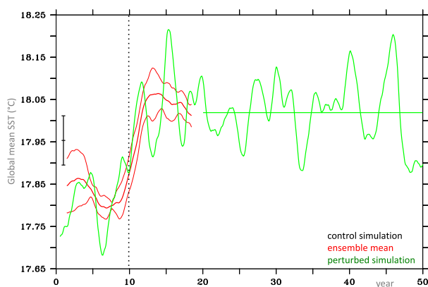
FIG. 7. Ensemble mean global mean SST ( ^{\circ}\text{C} ; thick red line) and \pm 1 ensemble standard deviation (thin red lines). The green line shows global mean SST for an individual ensemble member run out for 50 years. Monthly means are plotted, and a 36-month boxcar filter is applied to smooth the data. The vertical black line at the left is centered on the 140-yr mean value from the control simulation and indicates \pm 1 standard deviations (or \pm 2 standard errors). The dotted vertical line separates the hiatus period (years 1–10; doubled vertical diffusivity) from the surge period (years 11–20; standard vertical diffusivity).
