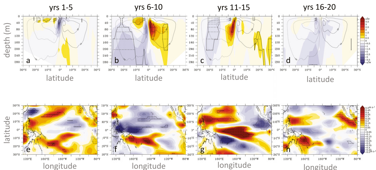
FIG. 15. Ensemble mean anomalous (top) overturning streamfunction (Sv) and (bottom) zonal wind ( \text{ms}^{-1} ) in the tropics (color shading) for (a),(e) years 1–5, (b),(f) years 6–10, (c),(g) years 11–15, and (d),(h) years 16–20. The thick black contours and dotted regions denote anomalies that are significantly different from the control simulation at the 95% confidence level. The thin black contours in (a)–(d) denote the control mean streamfunction (Sv).
