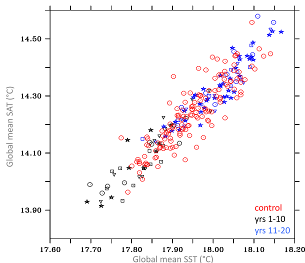
FIG. 8. Scatterplot of global annual mean SAT vs SST ( ^{\circ}\text{C} ) for control (red circles), hiatus period (years 1–10 of the ensemble experiment; black symbols) and surge period (years 11–20 of the ensemble experiment; blue symbols). Individual ensemble members are differentiated by different symbols: circles, stars, squares, and triangles.
