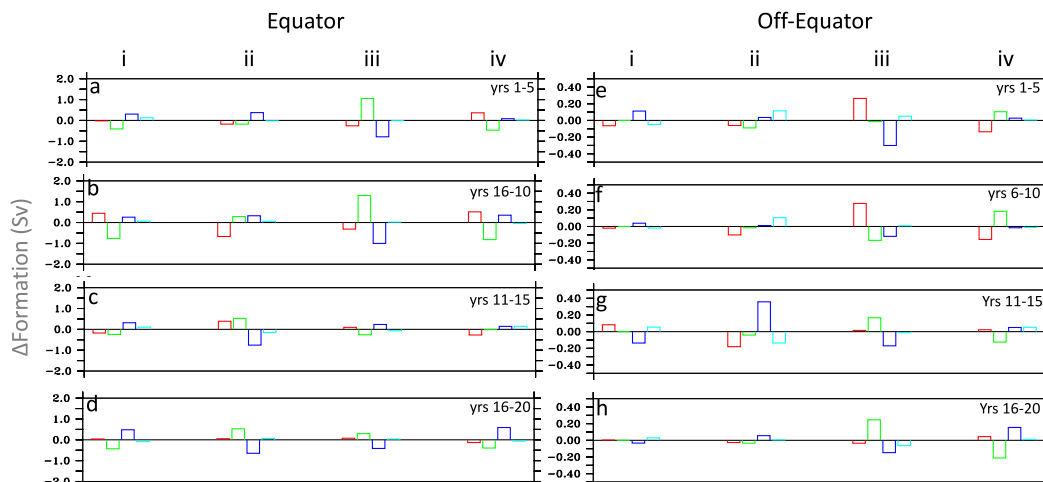
FIG. 14. Ensemble mean anomalous formation rate (Sv per degree of latitude) (left) at the equator (3°S–3°N) and (right) for the off-equatorial regions (average of 18°–12°S and 12°–18°N) associated with overturning (red), surface heat flux (green), mixing (blue), and volume change (cyan) for the four thermodynamic regimes (i–iv) defined in Fig. 10, for (a),(e) years 1–5, (b),(f) years 6–10, (c),(g) years 11–15, and (d),(h) years 16–20.
