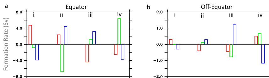
FIG. 11. Formation rate (Sv per degree of latitude) (a) at the equator (3°S–3°N) and (b) for the off-equatorial regions (average of 18°–12°S and 12°–18°N) in the control simulation associated with overturning (red), surface heat flux (green), and mixing (blue) for the four thermal regimes (i–iv) defined in Fig. 10.
