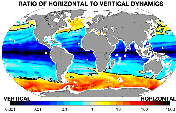
FIG. 4. Ratio of horizontal to vertical dynamics in log scale, following (15). The ratio ( \epsilon ) measures the propensity of the advection equation to be dominated by horizontal advection ( \epsilon \gg 1 ) or by vertical advection ( \epsilon \ll 1 ) under the geostrophic balance assumption. The former regime is more inductive to baroclinic instabilities, whereas the latter regime is more inductive to baroclinic Rossby waves. The thick black contour corresponds to the perfect balance (i.e., \epsilon = 1 ).
