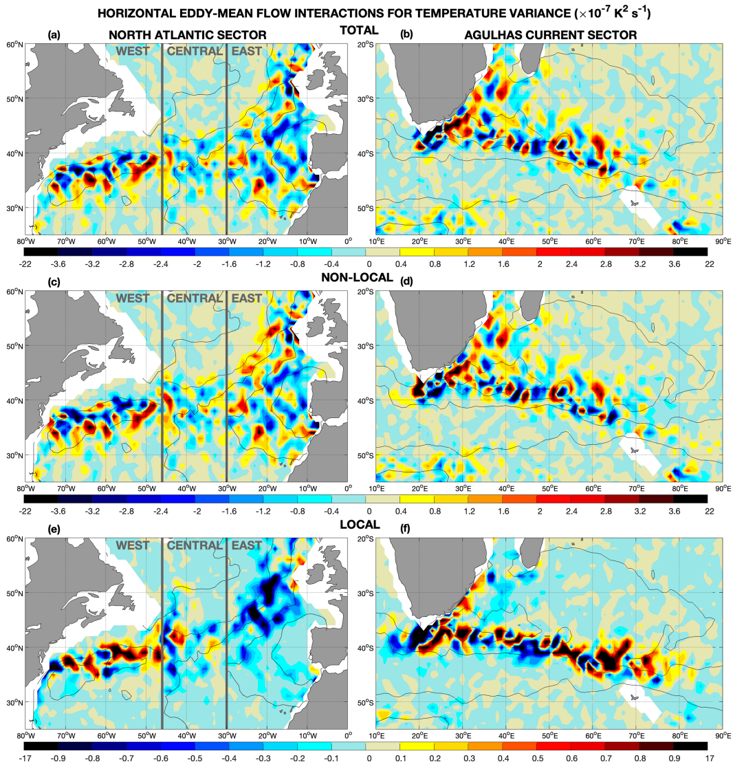
FIG. 9. As in Fig. 8, but zoomed for two key regions: (a),(c),(e) the west and east North Atlantic sectors and (b),(d),(f) the Agulhas Current sector. Components of the horizontal eddy-mean interactions for the temperature variance: (a),(b) total ( \mathcal{R}_{\text{hor}} ), (c),(d) nonlocal ( \mathcal{A}_{\text{hor}} ), and (e),(f) local ( \mathcal{T}_{\text{hor}} ), following (12). Positive and negative values correspond to variance transfers from ETV to MTV and from MTV to ETV, respectively. Contours show Conservative Temperature with contours from -2^\circ to 13^\circ\text{C} with a 1.5^\circ contour interval.
