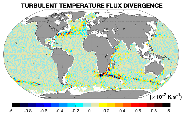
FIG. 7. Horizontal divergence of the horizontal turbulent temperature flux ( \mathcal{C}_{\text{hor}} = -\nabla_H^T \cdot \overline{\mathbf{u}_H' T'} ). This term corresponds to the horizontal components of the closure term (i.e., the impact of turbulence) for the mean temperature, following (6a).
