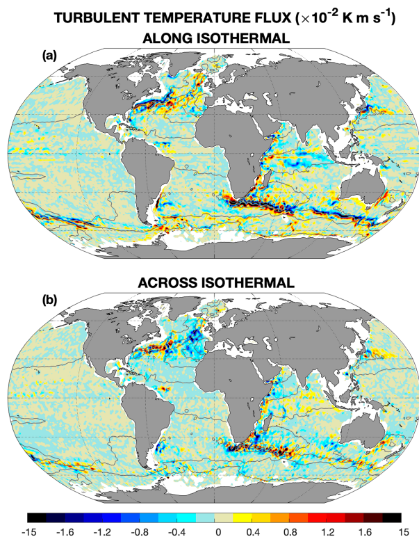
FIG. 6. Horizontal turbulent temperature flux. Flux projected (a) along conservative isotherms ( \overline{\mathbf{u}_H' T'}|_{\parallel} ) and (b) across conservative isotherms ( \overline{\mathbf{u}_H' T'}|_{\perp} ), following (16). Contours show mean Conservative Temperature with contours from -2^\circ to 13^\circ\text{C} with a 1.5^\circ contour interval.
