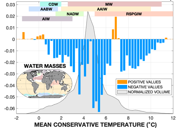
FIG. 10. As in Fig. 8c, but as a distribution in terms of Conservative Temperature classes, following (17). This corresponds to the distribution of local eddy-mean interactions for the temperature variance ( T|_{\text{hor}} ), following (12), as a function of the mean temperature. Positive (orange) and negative (cyan) values correspond to variance transfers from ETV to MTV and from MTV to ETV, respectively. The relative volume of each water class is given by the gray patch. Temperature classes are spaced by 0.25^\circ\text{C} , and the volume curves have been smoothed using a 1^\circ\text{C} moving average. The horizontal color patches show properties of selected water masses: AABW, CDW, AAIW, RSPGIW, MW, NADW, and the AIW, following Emery (2018). These water-mass locations are depicted in the inset.
