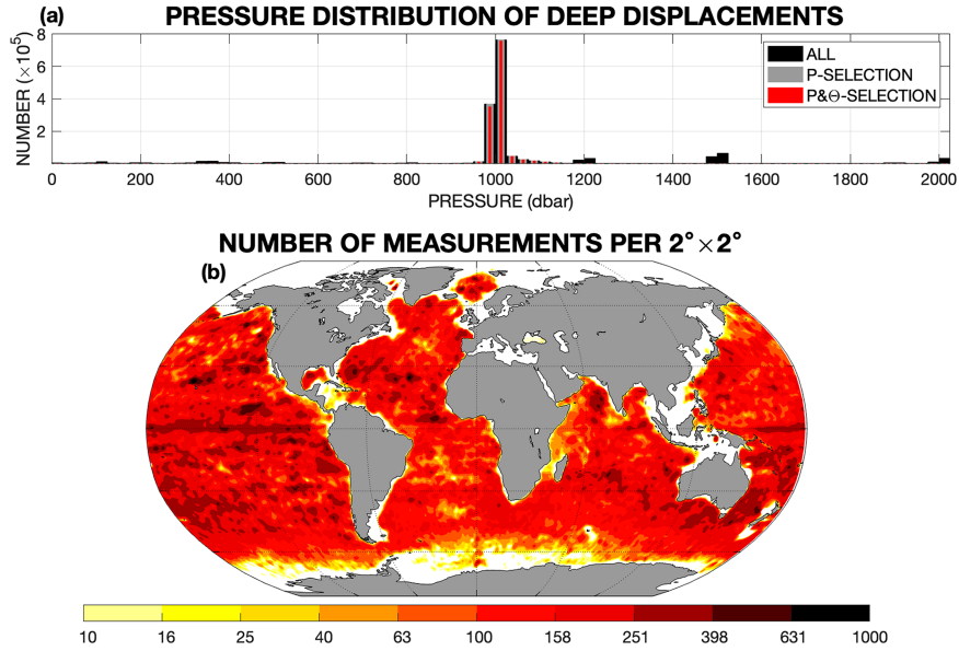
FIG. 1. Distribution of velocity observations from the ANDRO dataset. (a) Distributions of the parking depth pressure of the Argo float deep displacements from the ANDRO dataset (#116520). Two sequential selections of observations: “ P -selection” corresponding to a range of pressure (from 950 to 1150 dbar) and “ P & Θ -selection” corresponding to both the range of pressure and a range of Conservative Temperature (from -2^{\circ} to 13^{\circ}\text{C} ). (b) Number of P & Θ -selected deep velocity observations per 2^{\circ} \times 2^{\circ} . Note the logarithmic color scale.
