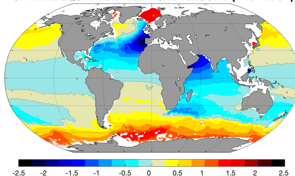
FIG. 11. Optimal equivalent vertical velocity, following (18). This vertical velocity leads to the most efficient mean vertical advection allowing for a global compensation of the variance transfer ( T ). (Note that, even at equilibrium, there is no need for a perfect local compensation, since advection can transport variance from local sources to local sinks.) Gray contour shows Conservative Temperature of \langle \Theta \rangle_{\text{hor}} \simeq 4.36^\circ\text{C} and perfectly matches \bar{w}_{\text{opt}} = 0 by construction of the anomalous Conservative Temperature (i.e., T = \Theta - \langle \Theta \rangle_{\text{hor}} ).
