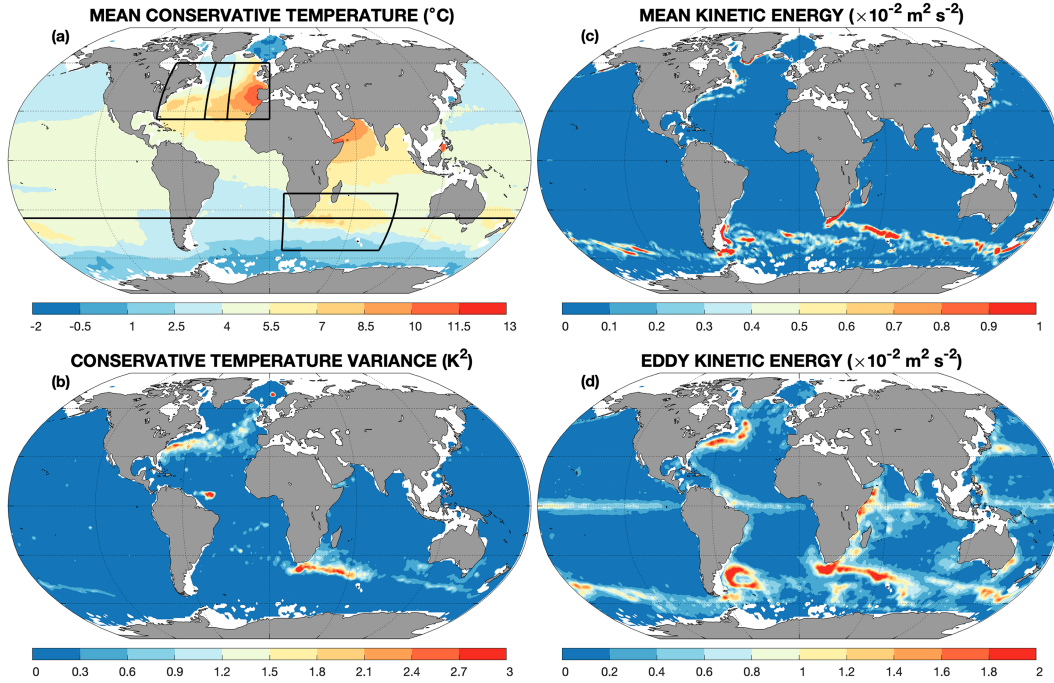
FIG. 2. Conservative Temperature and kinetic energy from Argo float deep displacement observations at 1000-m depth. (a) Mean Conservative Temperature ( \bar{\Theta} ), (b) Conservative Temperature variance ( \bar{\Theta}'^2 ), (c) MKE [ \text{MKE} = (\bar{u}^2 + \bar{v}^2)/2 ], and (d) EKE [ \text{EKE} = (\bar{u}'^2 + \bar{v}'^2)/2 ]. The observations have been mapped following (2) and (3). The black line and boxes denote the regions used for spatial averages: west, central, east, and all North Atlantic, Agulhas Current sector, and Southern Ocean sector.
