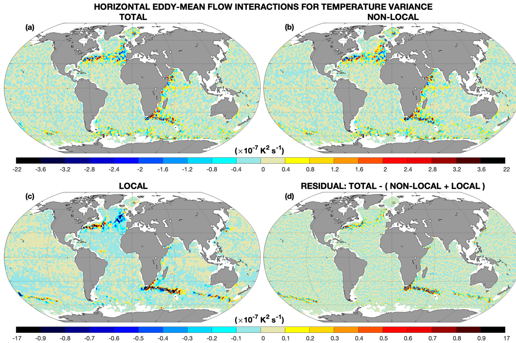
FIG. 8. Components of the horizontal eddy–mean interactions for the temperature variance: (a) total ( \mathcal{R}|_{\text{hor}} ), (b) nonlocal ( \mathcal{A}|_{\text{hor}} ), (c) local ( T|_{\text{hor}} ), and (d) residual ( \mathcal{R}|_{\text{hor}} - \mathcal{A}|_{\text{hor}} - T|_{\text{hor}} ), following (12). The residual should be equal to 0 and so measures the estimation error of the eddy–mean interactions. Note the different color scales for (a) and (b) vs (c) and (d). Positive and negative values correspond to variance transfers from ETV to MTV and from MTV to ETV, respectively.
