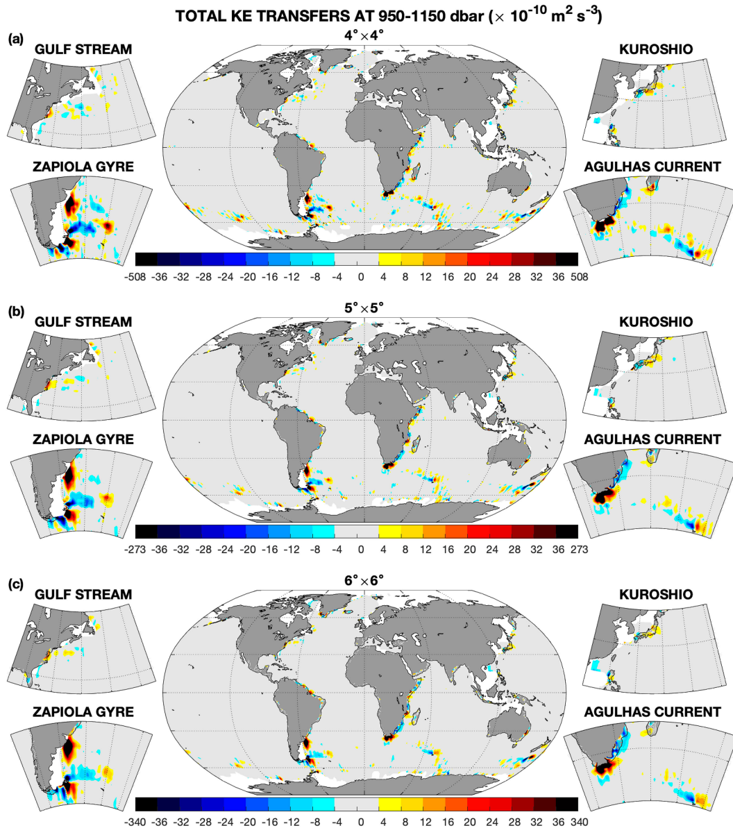
FIG. 14. Sensitivity of total MKE-to-EKE transfers to gridcell size. As in Fig. 4, but for flow statistics computed using (a) 4^\circ \times 4^\circ , (b) 5^\circ \times 5^\circ , and (c) 6^\circ \times 6^\circ cells.
