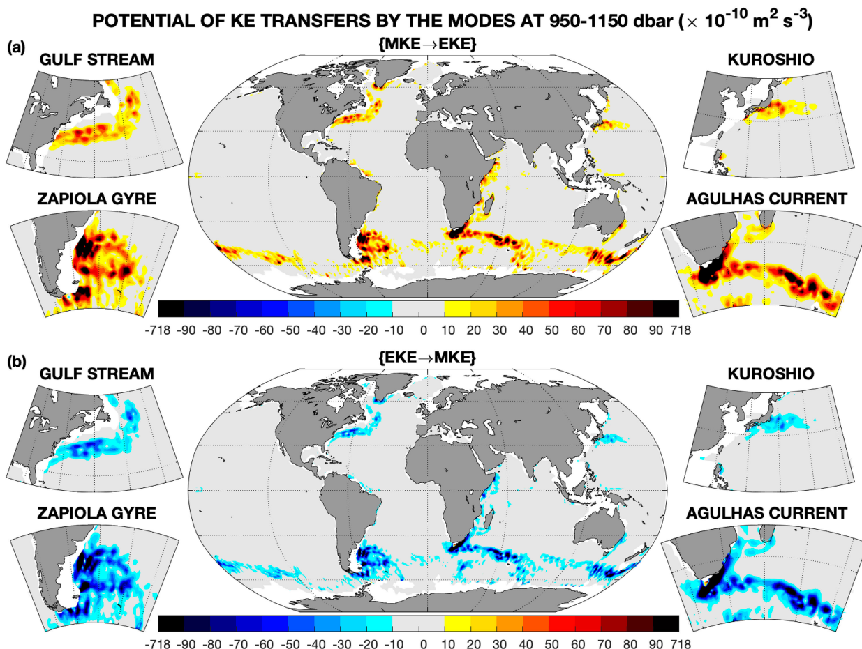
FIG. 12. Potential of MKE-to-EKE and EKE-to-MKE transfers. (a) Potential of MKE-to-EKE transfers ( \bar{\Phi}_{\{\text{MKE} \rightarrow \text{EKE}\}} ) and (b) potential of EKE-to-MKE transfers ( \bar{\Phi}_{\{\text{EKE} \rightarrow \text{MKE}\}} ), following (20). Positive and negative values show MKE-to-EKE and EKE-to-MKE transfers, respectively. Insets (clockwise from top left) show magnification for the Gulf Stream, Kuroshio, Agulhas Current, and Zapiola Gyre regions.
