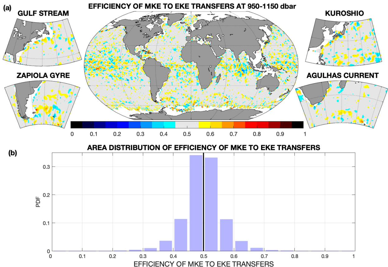
FIG. 13. Efficiency of MKE-to-EKE transfers. (a) Geographical map and (b) distribution of the efficiency of MKE-to-EKE transfers ( \bar{T}_{\{MKE \rightarrow EKE\}} ), respectively, following (21a). Values above or below 0.5 show regions more favorable to MKE-to-EKE or EKE-to-MKE transfers, respectively. Value 0 or 1 shows region purely following EKE-to-MKE or MKE-to-EKE transfers, respectively. Insets in (a) (clockwise from top left) show magnification for the Gulf Stream, Kuroshio, Agulhas Current, and Zapiola Gyre regions.
