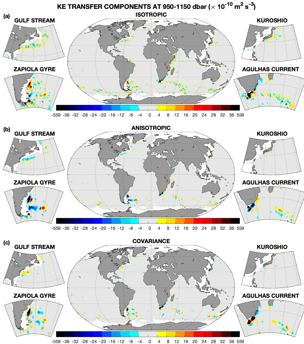
FIG. 6. Components of horizontal transfers of KE. As in Fig. 4, but for each of the KE transfer components of the decomposition (12), based on turbulent flow properties: (a) isotropic, (b) anisotropic, and (c) covariance components. Positive and negative values show MKE-to-EKE and EKE-to-MKE transfers, respectively. Insets (clockwise from top left) show magnification for the Gulf Stream, Kuroshio, Agulhas Current, and Zapiola Gyre regions.
