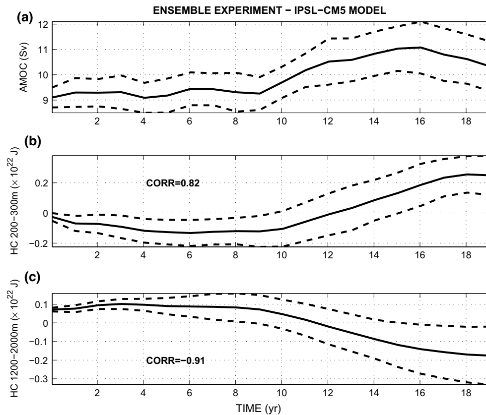
Fig. 7 Ensemble mean (solid line) and spread (dashed lines indicating the mean plus/minus one standard deviation) for a the AMOC intensity, b Ocean Heat Content (OHC) anomaly between 200 and 300 m, and c OHC anomaly between 1200 and 2000 m obtained in coupled climate simulations using the IPSL-CM5 model. The area of integration for OHC is from the equator to 60°N in the Atlantic. The two correlation coefficients shown are between the AMOC variations
