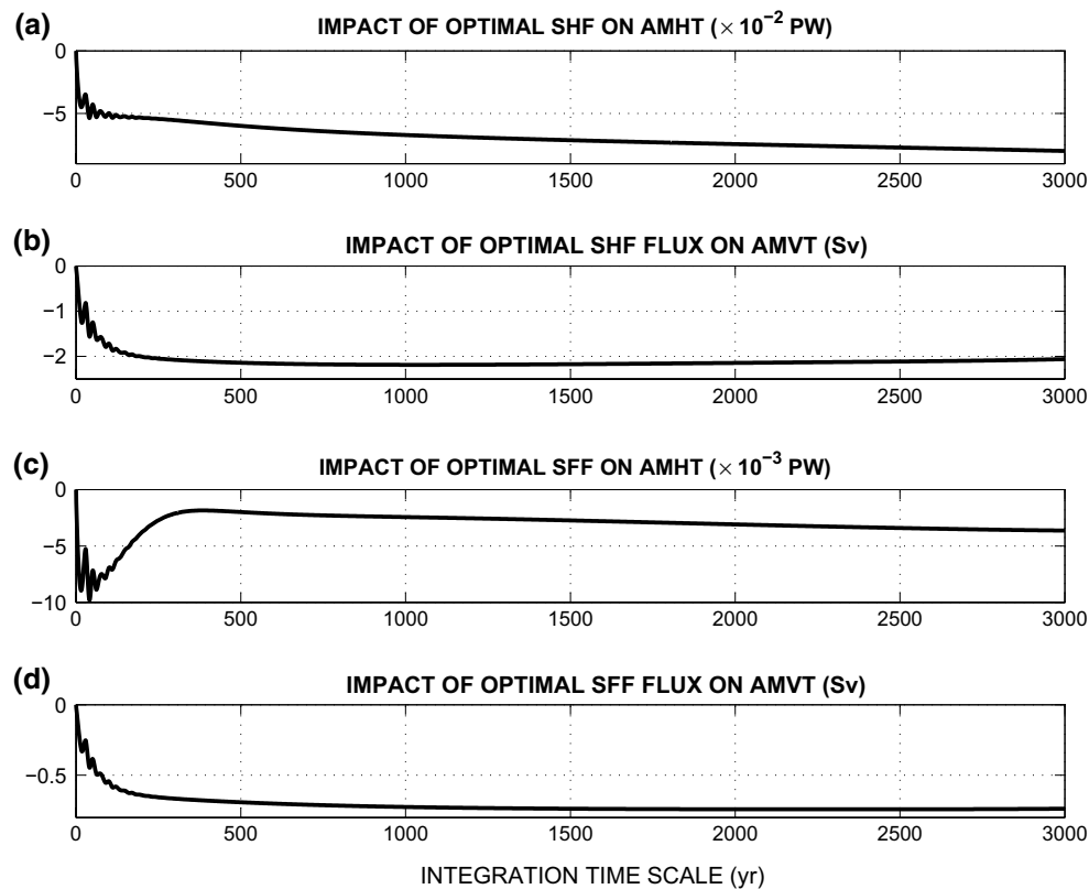
Fig. 2 The magnitude of impacts of surface a, b heat and c, d fresh-water fluxes that modify meridional a, c heat and b, d volume transports in the North Atlantic (AMHT and AMVT, respectively) most efficiently, as a function of integration timescale (i.e. corresponding to the duration of the imposed fluxes, \tau ). These results are obtained
