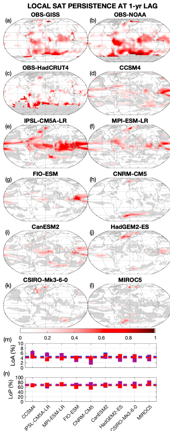
Figure 4. Local mean surface atmospheric temperature persistence in observations and CMIP5 models. Hindcasts are annually averages from 1881 to 2004 with a lag of 1 year. Surface Atmospheric Temperature persistence hindcast skills in (a–c) three observation data sets and (d–l) nine CMIP5 climate models (as the ensemble mean of member persistence). Gray indicates insufficient data for observations and a higher standard deviation than mean for models. (m) Level of Agreement (LoA) measures the relative area of the globe for which the models reproduces the observation persistence skills within a relative error of \pm 10\% . (n) Level of Paradox (LoP) measures the relative area of the globe where the paradox occurs (i.e., weaker persistence skills in models than in observations). Red, purple, and blue indicate model comparisons with the GISS, NOAA, and HadCRUT4 observation data sets, respectively. Models have been sorted from the closest to observations to further away, over the 5-year time lags tested for GMT (following Figure 3).
