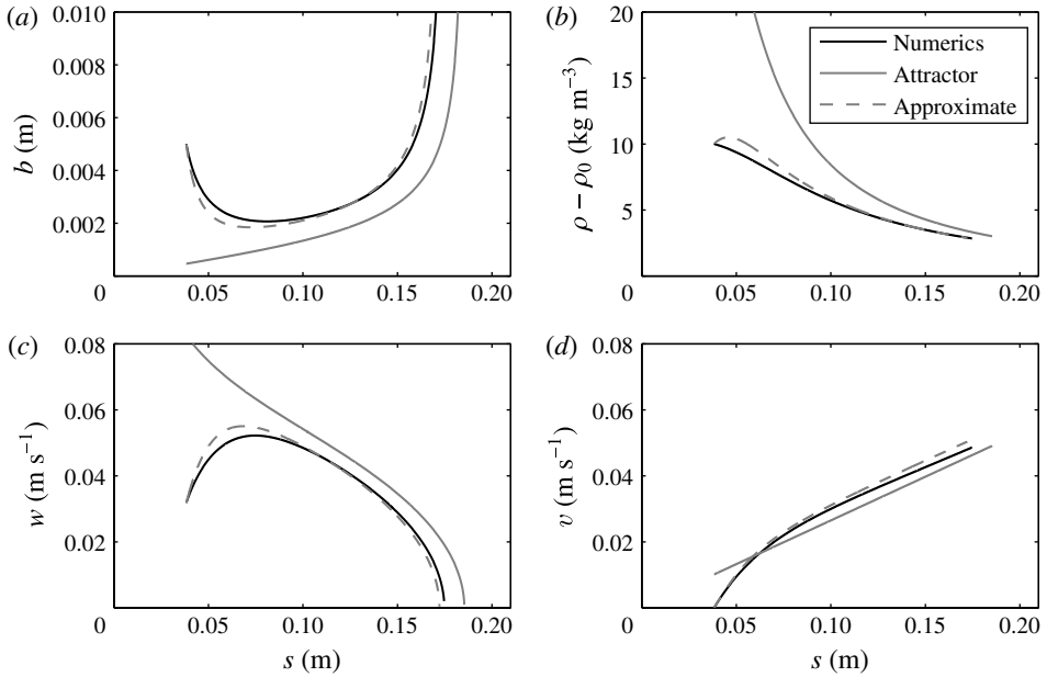
FIGURE 2. Flow development with distance s from the apex of the cone: (a) thickness; (b) density anomaly; (c) downslope velocity; (d) azimuthal velocity. The thick black solid curves represent the numerical solution of the full equation set (2.1)–(2.10), whilst thin grey curves show the asymptotic attractor solution (3.10)–(3.12) and dashed curves show the approximate solution including higher-order corrections (3.14) and (3.19)–(3.21). The downslope flow ceases at a critical point s_{cr} where w \rightarrow 0 , b \rightarrow \infty and the boundary layer approximation breaks down. The parameters used are representative of a laboratory experimental set-up, with g = 9.8 \text{ m s}^{-2} , \rho_o = 1000 \text{ kg m}^{-3} , \Omega = 0.6 \text{ rad s}^{-1} and \alpha = 36^\circ , and for illustration we set E = 0.1 \sin \alpha (Wells & Wettlaufer 2005) and K = 2 \times 10^{-3} , consistent with the order of magnitude determined by Taylor (1920). The prescribed initial conditions at s = 0.038 \text{ m} are \rho = 1010 \text{ kg m}^{-3} , b = 5 \times 10^{-3} \text{ m} , w = 3.2 \times 10^{-2} \text{ m s}^{-1} and v = 0 \text{ m s}^{-1} .
