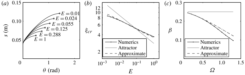
FIGURE 3. (a) Fluid parcel trajectories s(\theta) from numerical solutions for a range of entrainment coefficients E , with \Omega = 1 rad s -1 and all remaining parameters as in figure 2; circles denote the critical points achieved at the end of the trajectories. (b) Sensitivity of the non-dimensional critical point \xi_{cr} = s_{cr} f^{3/4} Q_B^{-1/4} to the entrainment coefficient E , plotted for \Omega = 1 rad s -1 ; the numerical solution (thick black solid curve) is compared with the analytical scaling (3.22) for the attractor (thin grey curve) and the approximate solution (dashed curve) with higher-order corrections (3.14) and (3.19)–(3.21); note the logarithmic scales. (c) Approximate power-law exponent \beta plotted as a function of \Omega (rad s -1 ), where \beta is estimated from a power-law fit \xi_{cr} = A E^{-\beta} to the curves in (b) and similar curves with different rotation rates, to approximate the sensitivity of the critical distance to entrainment; the numerical solution converges toward the attractor at small \Omega .
