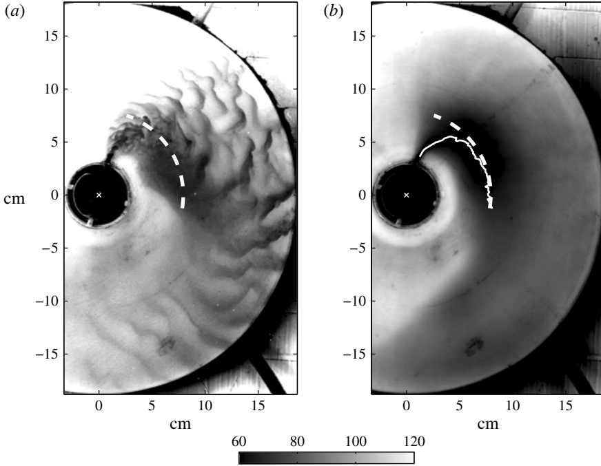
FIGURE 4. (a) A top-view snapshot of the single-stream density current for experiment no. 10 listed in table 1. (b) A corresponding image temporally averaged over 10 inertial periods. The scale shows the greyscale pixel intensity in the digital images, with regions of higher concentration of the dyed fluid in the descending dense current having darker intensity. Overlaid are the centre-line trajectory (white solid curve) and a critical level indicated by a white dashed circular arc with radius R_{cr} ; the white cross in each panel denotes the axis of rotation.
