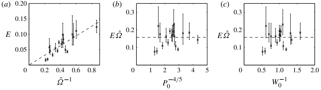
FIGURE 7. Investigation of the scaling of the entrainment rate E with the dimensionless groups \hat{\Omega} = fs_l^{4/3} Q_B^{-1/3} , P_0 and W_0 defined by (3.2), which depend on the rotation rate f : (a) variation of the scaled entrainment rate E with \hat{\Omega}^{-1} (crosses with error bars, as in figure 6), which is consistent with a fitted linear trend E = 0.16 \hat{\Omega}^{-1} , shown by the dashed line; (b) variation of the renormalised quantity E\hat{\Omega} with P_0^{-4/5} \propto 1/f (crosses with error bars); (c) variation of E\hat{\Omega} with W_0^{-1} \propto 1/f (crosses with error bars). Panels (b) and (c) indicate that the E = 0.21 \hat{\Omega}^{-1} trend (dashed line) captures the leading scaling with f , and there is no further systematic variation with the initial conditions P_0 or W_0 .
