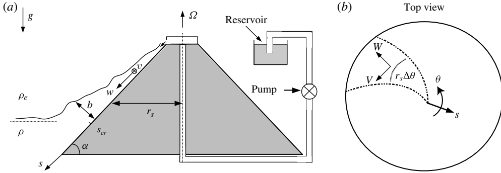
FIGURE 1. Schematic view of the density current on a cone in a rotating fluid, as described in the main text: (a) view from the side, indicating the system geometry, notation and experimental set-up; (b) view from above for a current with effective angular extent \Delta\theta .
