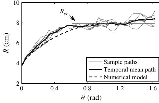
FIGURE 5. Reconstructed time-averaged trajectory given in polar form R(\theta) (solid black curve) for experiment no. 10 listed in table 1, along with sample trajectories indicating time variability (grey curves). The level of R_{cr} is plotted starting from the value of \theta at which the index I_w takes its first minimum (horizontal grey line). A numerical solution (dashed black curve) is obtained using the experimental initial conditions and the best-fit entrainment coefficient corresponding to the observed R_{cr} .
