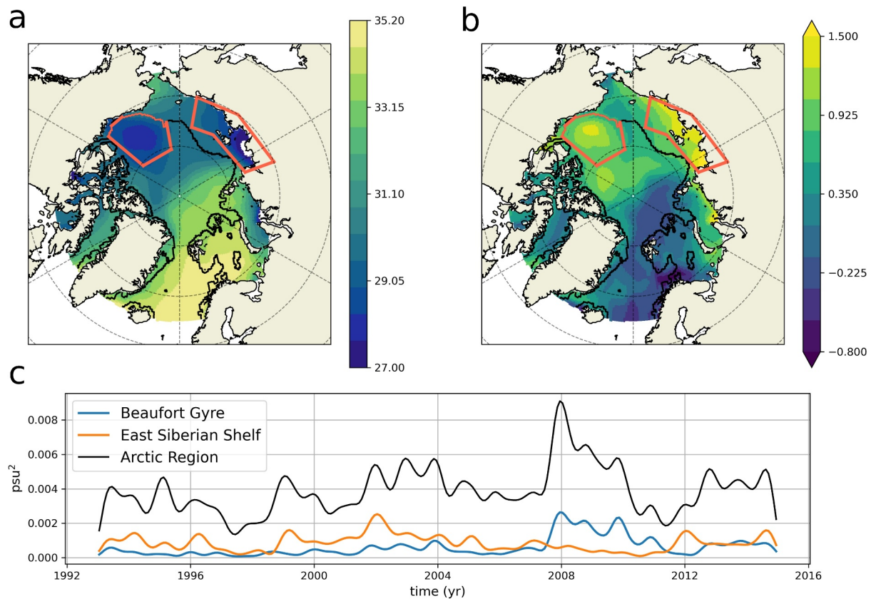
Figure 2. (a) Time mean surface salinity in the Arctic Basin (in psu) defined by latitudes North of 65^{\circ}\text{N} . (b) \log_{10} of the vertically integrated variance of the interannual salinity anomaly (in \text{psu}^2 \text{m} ) for the period 1993–2014. The two orange boxes show the location of the Beaufort Gyre (BG) and the East Siberian Shelf (ESS) boxes and the black contour shows the 300 m isobath. Panel (c): volume integral of the squared interannual salinity anomaly in the BG (blue line), ESS (orange line) and Arctic regions over the period 1993–2014. The three volume integrals are divided by the total Arctic volume.
