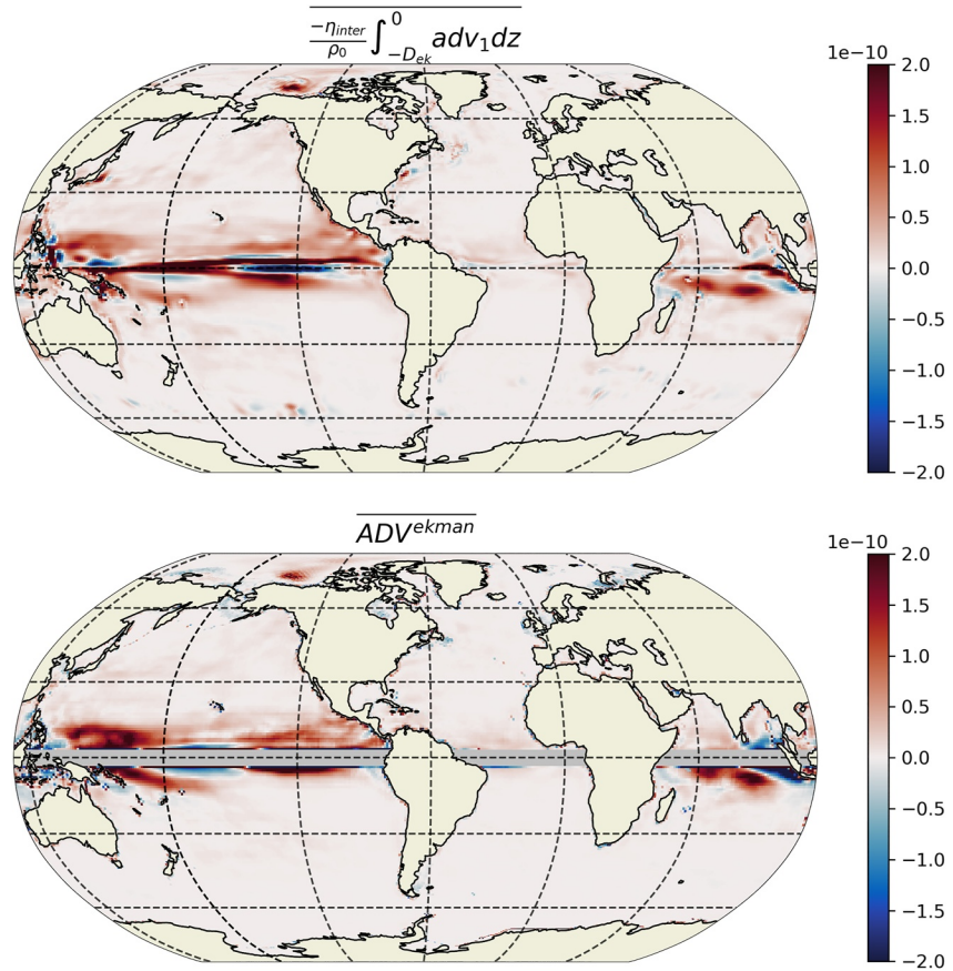
Figure 5. Top panel: same as \overline{ADV}_{steric}^1 (top panel, Figure 4) but where adv_1 is vertically integrated in the Ekman layer instead of over the full depth. Bottom panel: ADV^{Ekman} (in m^2 s^{-1} ): term associated with the advection of the mean density by 3D Ekman velocities, vertically integrated in the Ekman layer [see formula Equation 15]. The gray band close to the equator corresponds to the region where the Ekman balance does not hold.
