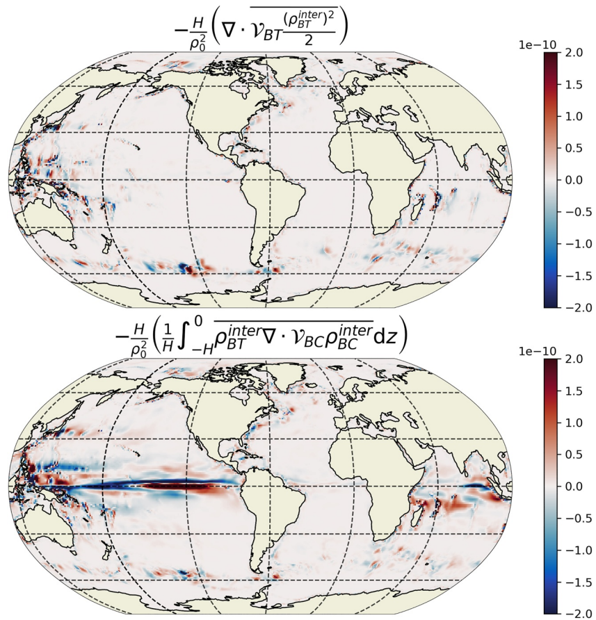
Figure 7. Decomposition of the sum of \overline{ADV^2_{steric}} + \overline{ADV^3_{steric}} (in m^2 s^{-1} ) as the sum of the convergence of interannual barotropic density variance due to mean and interannual velocities (top panel) and the transfer between the interannual barotropic and baroclinic density variance (bottom panel). The two corresponding formulas in Equation 31 have been rescaled by H\rho_0^2 (following Equation 24) for easier comparison with the steric sea level terms ADV^2_{steric} and ADV^3_{steric} from Figure 4.
