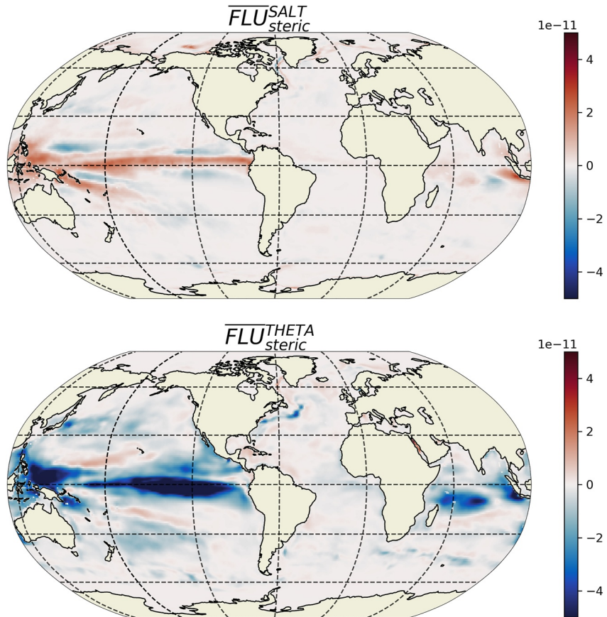
Figure 3. Decomposition of the atmospheric fluxes term ( \overline{\text{FLU}}_{\text{steric}} , in \text{m s}^{-2} ) into a part associated with salinity due freshwater fluxes (top panel) and a part associated with temperature and due to the net heat flux from the atmosphere (bottom panel). The spatial integral of the 2 terms is given in Table 1.
