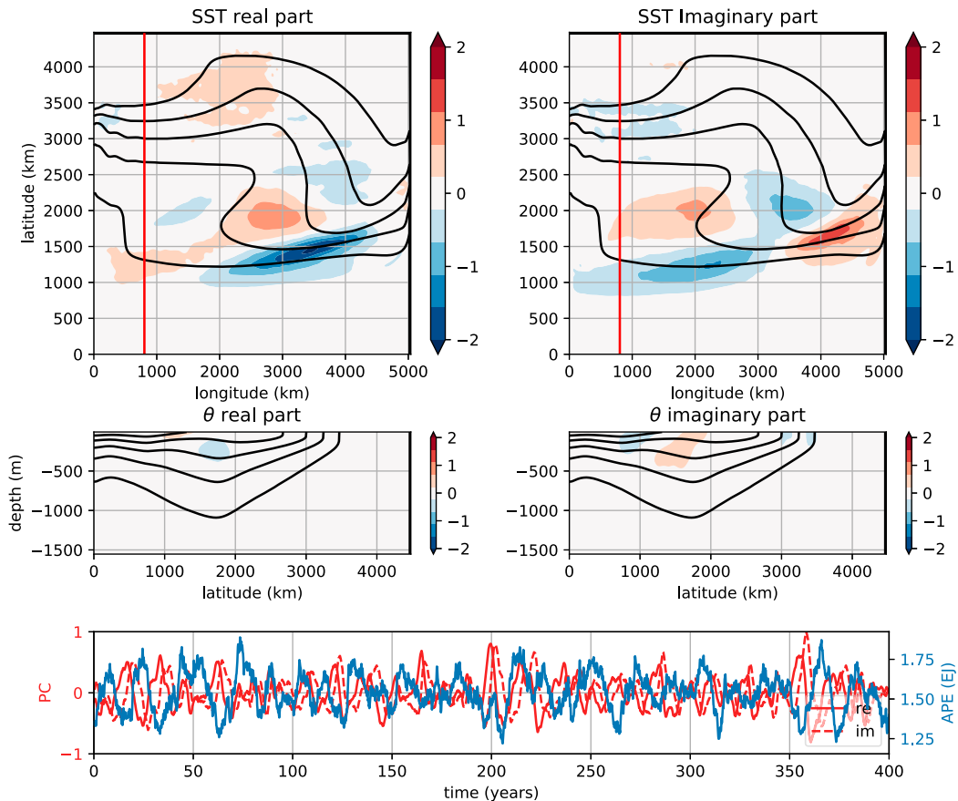
FIG. 9. As in Fig. 6, but for a climatological double-gyre wind forcing of \tau_0 = 0.1 \text{ N m}^{-2} . The leading CEOF accounts for 7% of the temperature variance.
