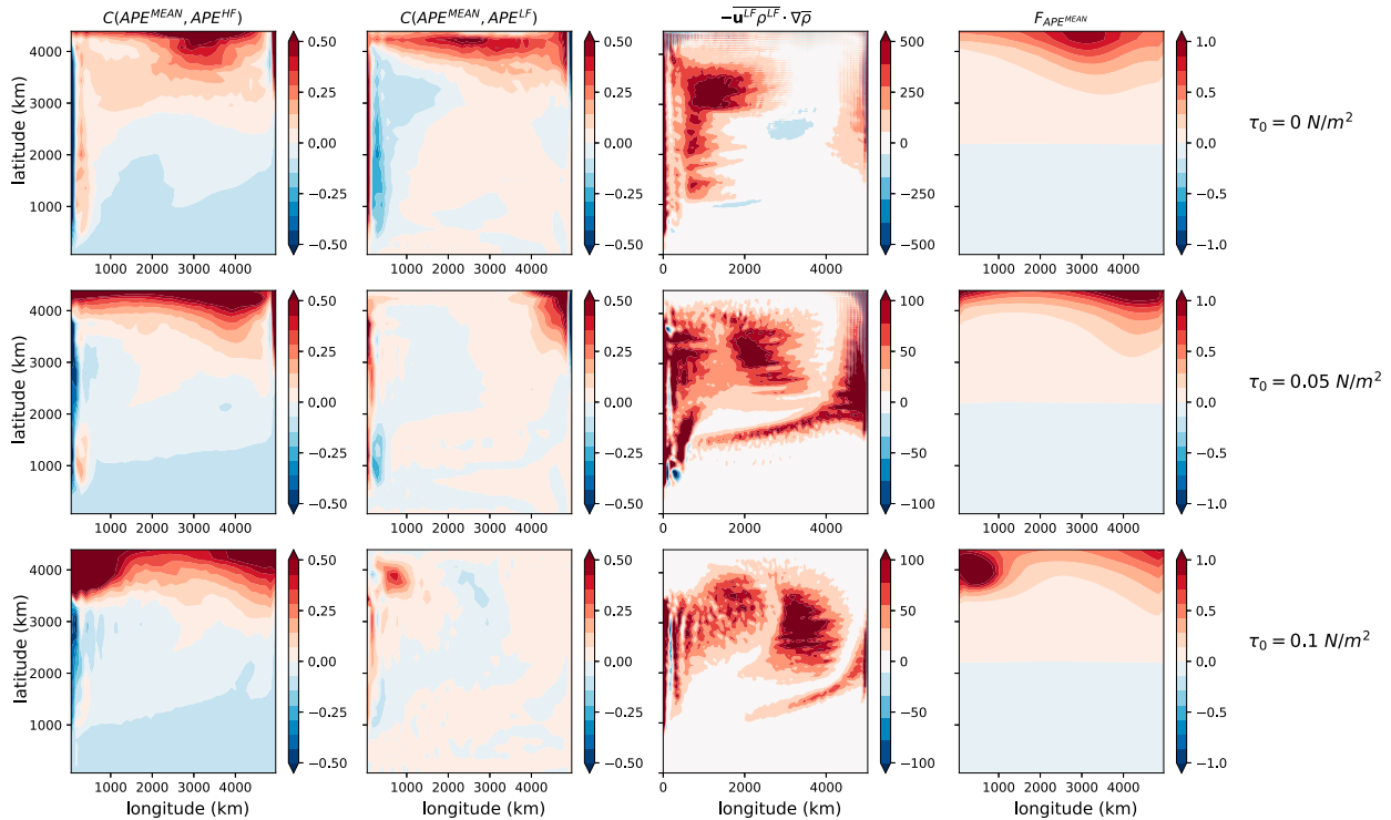
FIG. 11. Vertical integral of the conversion between (left) mean APE and HF APE [C(\text{APE}^{\text{MEAN}}, \text{APE}^{\text{HF}})] and (left center) mean APE and LF APE [C(\text{APE}^{\text{MEAN}}, \text{APE}^{\text{LF}})] (GW), (right center) the vertical integral of the density variance transfer from mean to LF (\text{kg}^2 \text{m}^{-6} \text{s}^{-1}) , note that the range of the color bar is different in the top panel), and (right) the mean APE forcing (or transfer from BPE to mean APE due to heat fluxes) (GW) for the three wind intensities (top) \tau_0 = 0 \text{ N m}^{-2} , (middle) \tau_0 = 0.05 \text{ N m}^{-2} , and (bottom) \tau_0 = 0.1 \text{ N m}^{-2} . Note that C(\text{APE}^{\text{LF}}, \text{APE}^{\text{HF}}) is not shown but looks very similar to C(\text{APE}^{\text{MEAN}}, \text{APE}^{\text{LF}}) .
