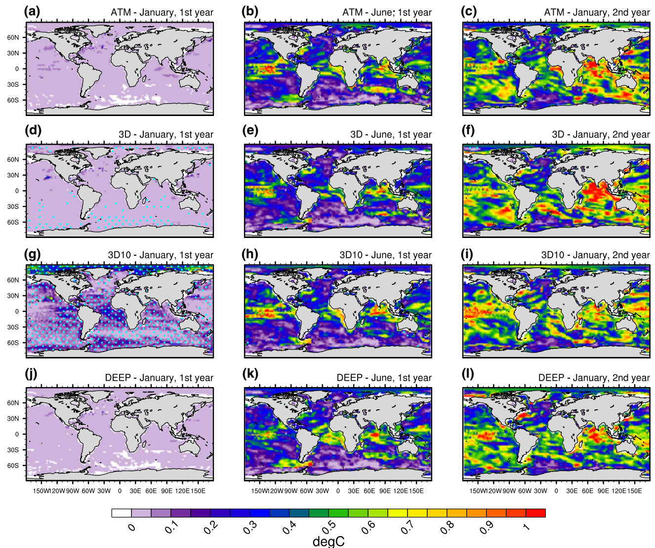
Fig. 6 ATM (1st row), 3D (2nd row), 3D10 (3rd row), and DEEP (4th row) ensemble spread of the oceanic temperature at 140 m depth at 1 (1st column), 6 (2nd column) and 13 (3rd column) months forecast. The ensemble spread is normed by the STD of January
