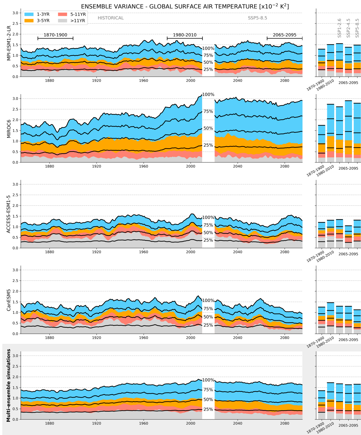
FIG. 1. Ensemble variance of globally averaged SAT. The four first rows show the ensemble variance for four different models: MPI-ESM1-2-LR, MIROC6, ACCESS-ESM1-5, and CanESM5. The last row presents the variance computed from a multiensemble constructed from the concatenation of the four previous models. (left) The yearly results for the historical and projected period with the Fossil-fueled Development scenario (SSP5-8.5). The colors represent the contribution of the various frequency bands to the total variance: blue for the variability with a period band of 1–3 years, orange for 3–5 years, red for 5–11 years, and gray for periods longer than 11 years. The bands are obtained from a temporal filtering of temperature at the given period, and all the bands of variance are finally filtered to be consistent with the 11-yr period. (right) The results for a given climatic period (averaged over 30 years): early historical (1870–1900), end of historical (1980–2010), and end of projections (2065–95) for three shared socioeconomic pathways: Sustainability (SSP1-2.6), Middle of the Road (SSP2-4.5), and Fossil-fueled Development (SSP5-8.5). The black lines represent the quarters of the total variance.
