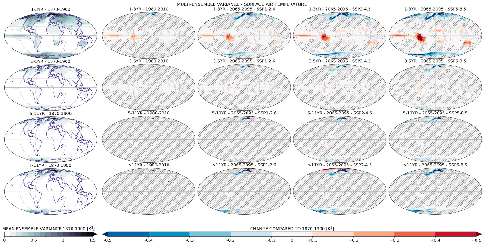
FIG. 3. Multiensemble variance of local SAT. Each column corresponds to a given 30-yr segment from the collection of four models assembled together. The first column is the ensemble variance for the early historical reference taken between 1870 and 1900. The four following columns show the deviation from this reference. The second column is the end of the historical period averaged between 1980 and 2010. The three last columns present projections of the same time period at the end of the projection runs (2065–95) for three shared socioeconomic pathways: Sustainability (SSP1-2.6), Middle of the Road (SSP2-4.5), and Fossil-fueled Development (SSP5-8.5). Each row corresponds to a given frequency band of the variability extracted from the time filtering of the variance signal: (row 1) 1–3 years, (row 2) 3–5 years, (row 3) 5–11 years, and (row 4) variability with period greater than 11 years. The gray hatched area corresponds to the area where the change in variance is not significant, i.e., where the signal-to-noise ratio of the variance is less than 1, where the 95% confidence interval associated with the change in variance is greater than the magnitude of that change.
