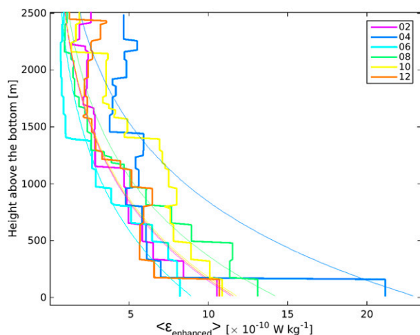
FIG. 7. Transect average of vertical dissipation rate profiles whose bottommost values are larger than 5 \times 10^{-10} \text{ W kg}^{-1} (thick lines). The average was computed as a function of height above the bottom. The color depicts the transect year and the thin line is a fit of an exponential profile decaying with a 1000-m vertical scale. Depending on the year, 8–12 profiles were averaged.
