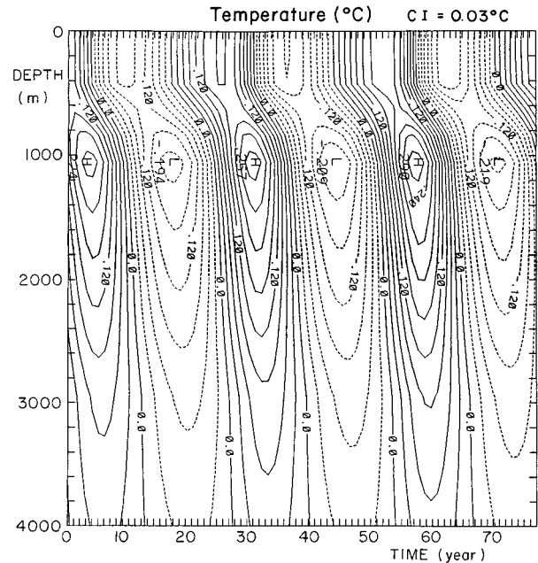
FIG. 6. Characteristic z-t diagram of the temperature field at a point situated in the unstable northwest corner region (LR run). The phase shift of the temperature distribution appears below the mixed layer.
