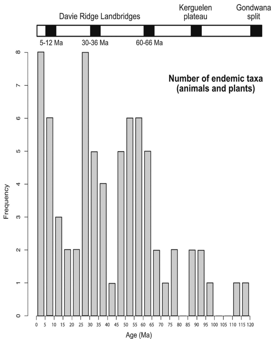
Fig. 3. Histogram showing the frequency distribution of the first occurrence of monophyletic endemic taxa in Madagascar through time. Data are given in supplementary material ( Table 1 ).
