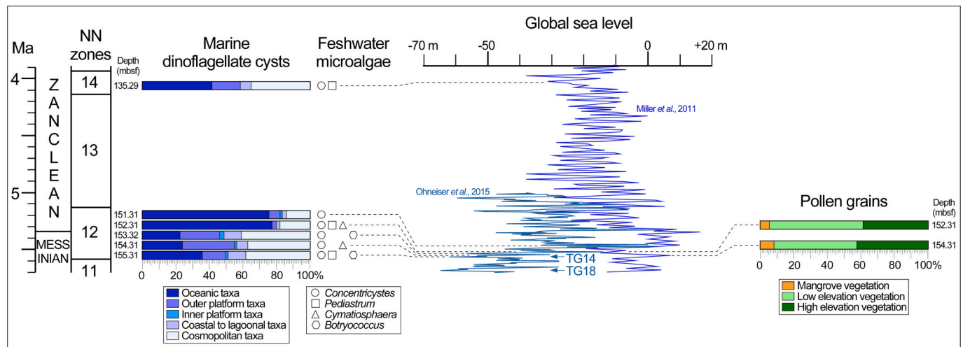
Fig. 4. DSDP Site 242: summary diagrams of marine dinoflagellate cyst and pollen grain assemblages grouped according to their origin and/or significance, including occurrence of four freshwater microalgae, and chronostratigraphically distributed with respect to biostratigraphy (calcareous nannoplankton) and global sea-level fluctuations (Miller et al., 2011 Vs. Ohneiser et al., 2015).
