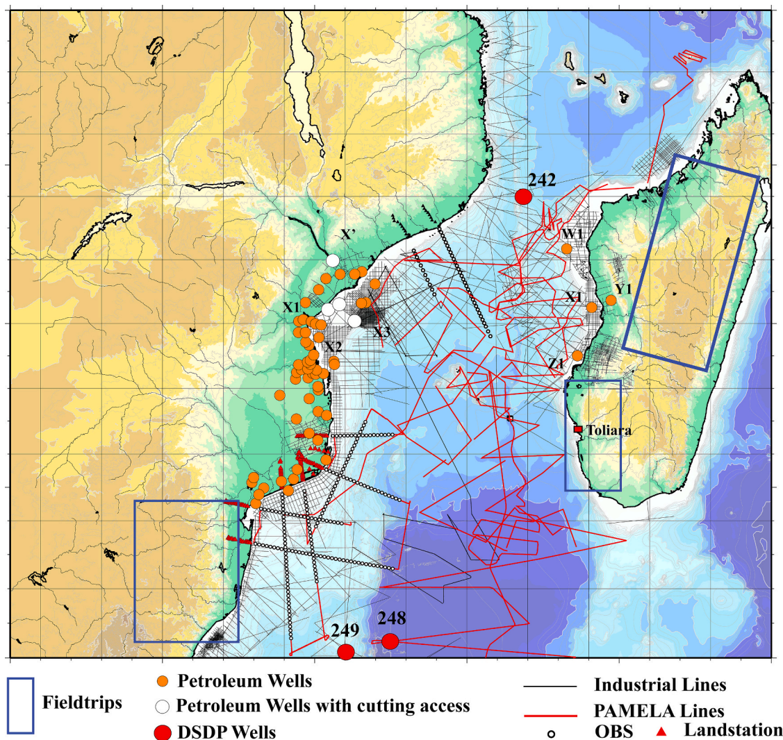
Fig. 1. Data used in the PAMELA Project used to reconstruct the palaeobathymetries of Masters et al. (2021) . Compilation after Ponte (2018) , Moulin et al. (2020) , Delaunay (2018) .
