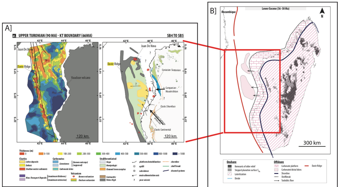
Fig. 2. A) Sediment thickness (isopach) maps and facies (palaeogeographic) map for the Upper Turonian (90 Ma) - KT boundary (66 Ma) depositional sequence. B) Synthetic map of the extension of the Lower Eocene (56-50 Ma) carbonate (after Delaunay, 2018 ). Net of other problems, note the difference between Delaunay's (2018) original interpretation of a highly continuous «palaeo-high» in the Sakalaves area and that of a strongly disrupted « seabed high », in the same area, given in Ali and Hedges's (2022) fig. 11 and allegedly attributed to Delaunay (2018) .
