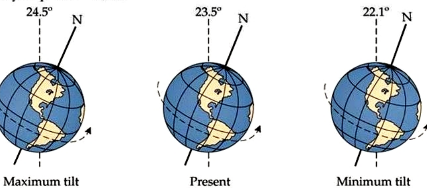
Milankovitch Cycles. Schematic of the Earth's orbital changes (Milankovitch cycles) that drive the ice age cycles. 'T' denotes changes in the tilt (or obliquity) of the Earth's axis, 'E' denotes changes in the eccentricity of the orbit (due to variations in the minor axis of the ellipse), and 'P' denotes precession, that is, changes in the direction of the axis tilt at a given point of the orbit. Source: Rahmstorf and Schellnhuber (2006).
