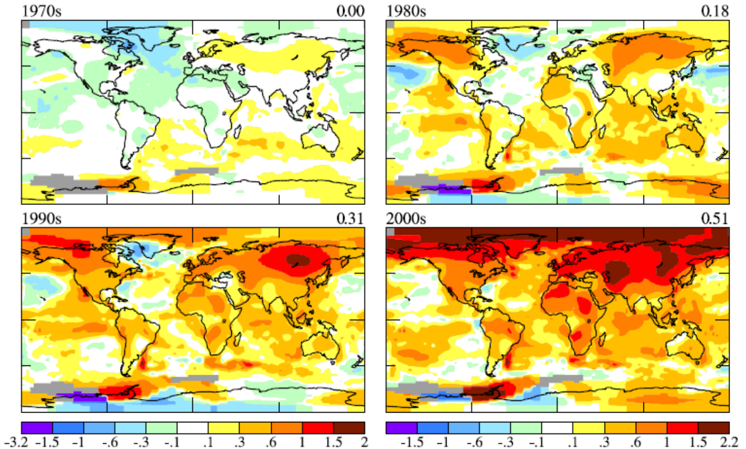
Decadal Surface Temperature Anomalies (°C)
