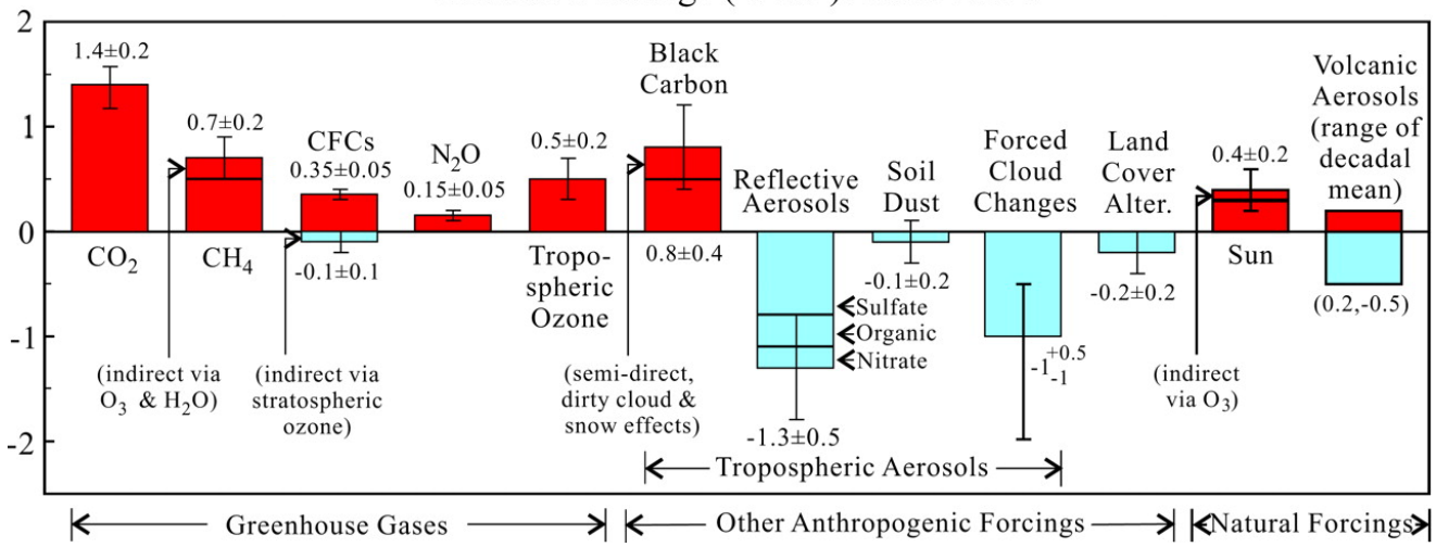
Climate Forcings ( W/m^2 ): 1850-2000
