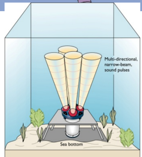
(b) DOPPLER ACOUSTIC CURRENT METER
